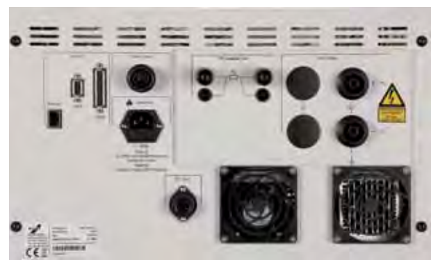
Rear view F7-1C; F7-1P
